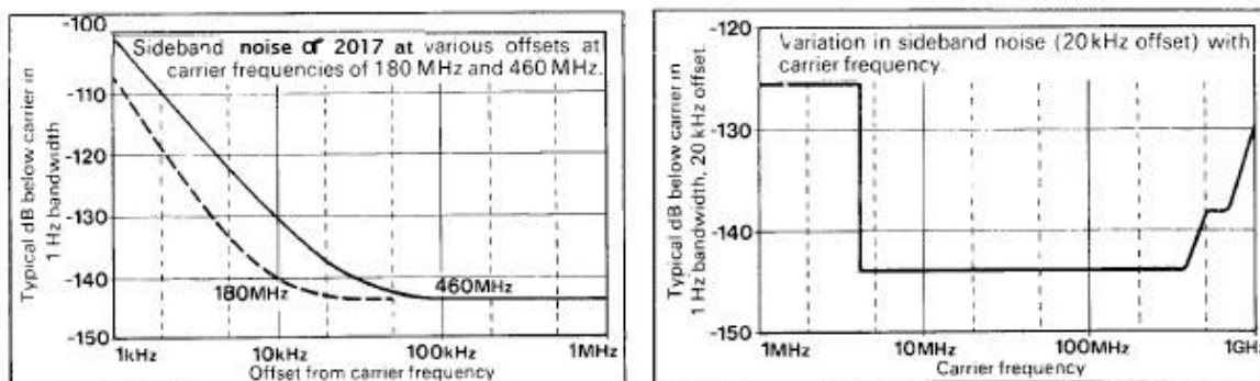
Fig. 2 Sideband noise curves
