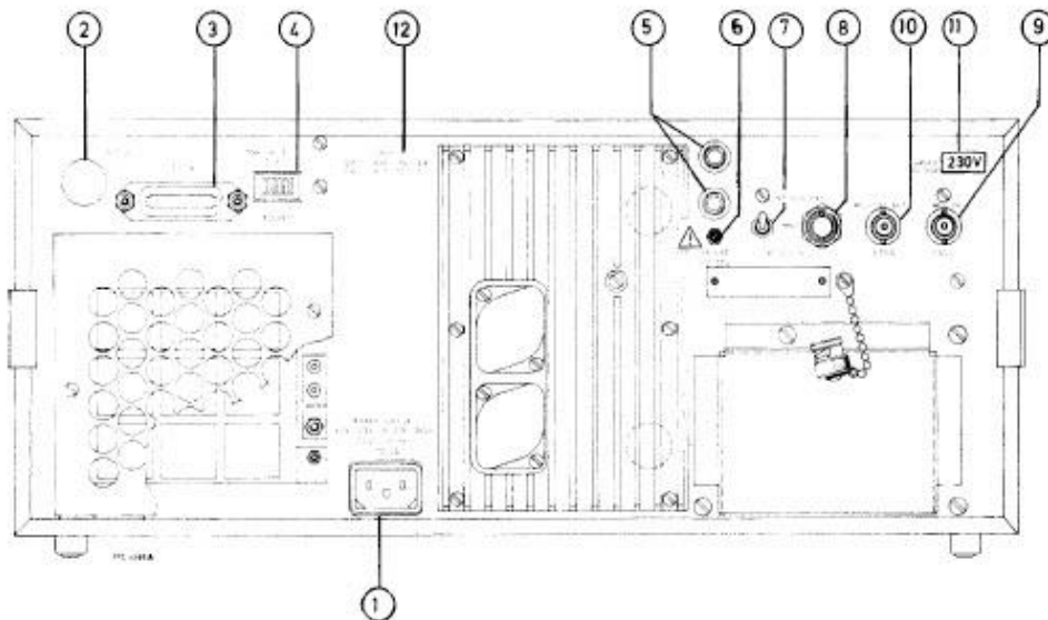
Fig. 2 Rear panel controls
