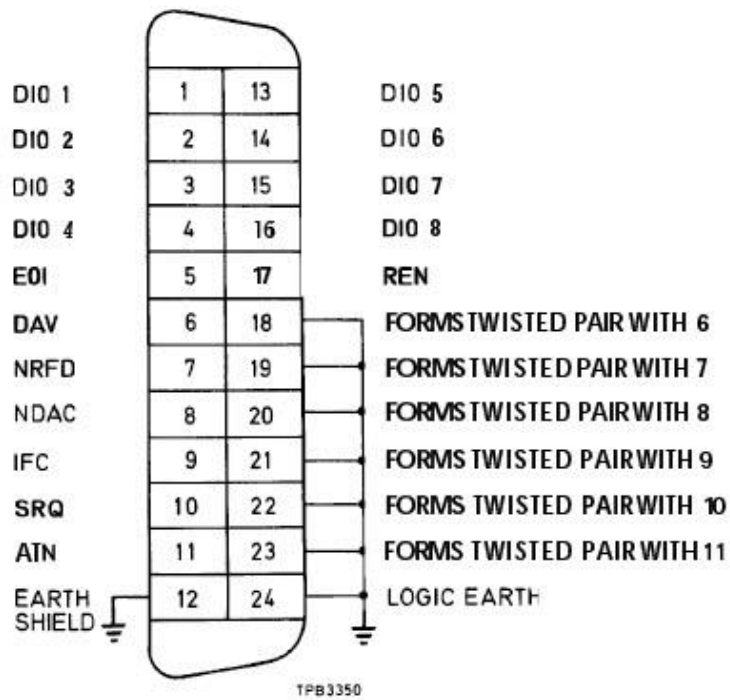
Fig. 3 GPIB connector contact assignments
